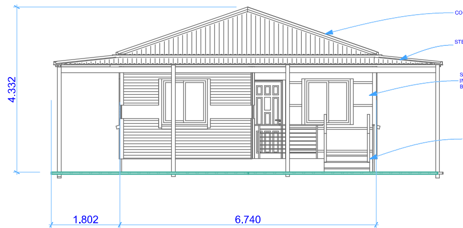
S-06 ELEVATIONS 1:100
